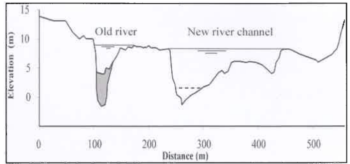
Above: Bellingher River channel size at Bellingher Island The old river channel was narrow and deep, the new channel is shallower and broader.
